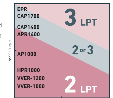
LPT cylinders application chart for 1880™ LSB *NSSS: Nuclear Steam Supply System
