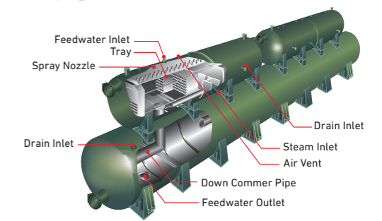
Double-Shell Type Deaerator
